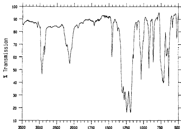
Figure 1. FTIR spectrum in \text{CH}_2\text{Cl}_2 of the trifluoromethanesulfonate salt of the in -bicyclo[4.4.4]tetradecyl cation 3.
