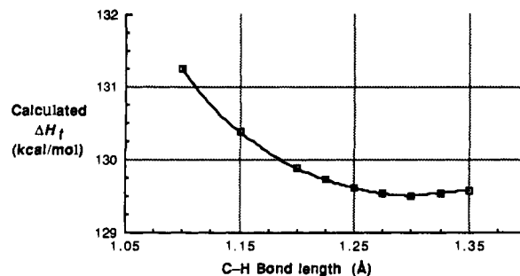
Figure 2. Plot of C-H bond length versus calculated (AM1) heat of formation for the C-H-C three-center bond in in -bicyclo[4.4.4]tetradecyl cation 3.
