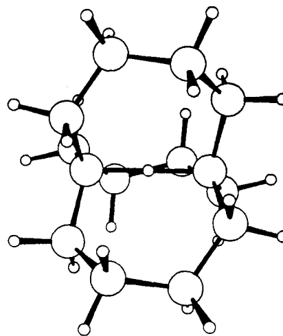
Figure 3. Computer-generated structure of the in -bicyclo[4.4.4]-1-tetradecyl cation using coordinates derived from semiempirical calculations.
